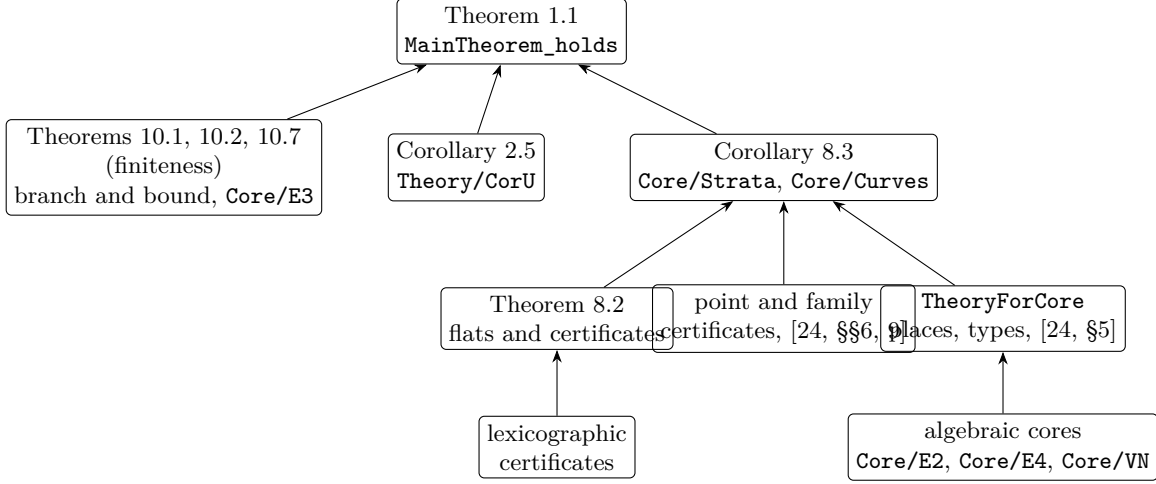
FIGURE 1. The main dependencies of the formal proof. An arrow points from a result to a result that uses it.
