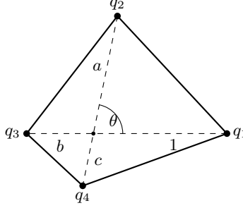
Fig. 1. The coordinates of [9], drawn at a = 0.9 , b = 0.5 , c = 0.4 and x = \cos \theta = 0.2 , a point where all six g_i are positive. The diagonals meet at the origin.
