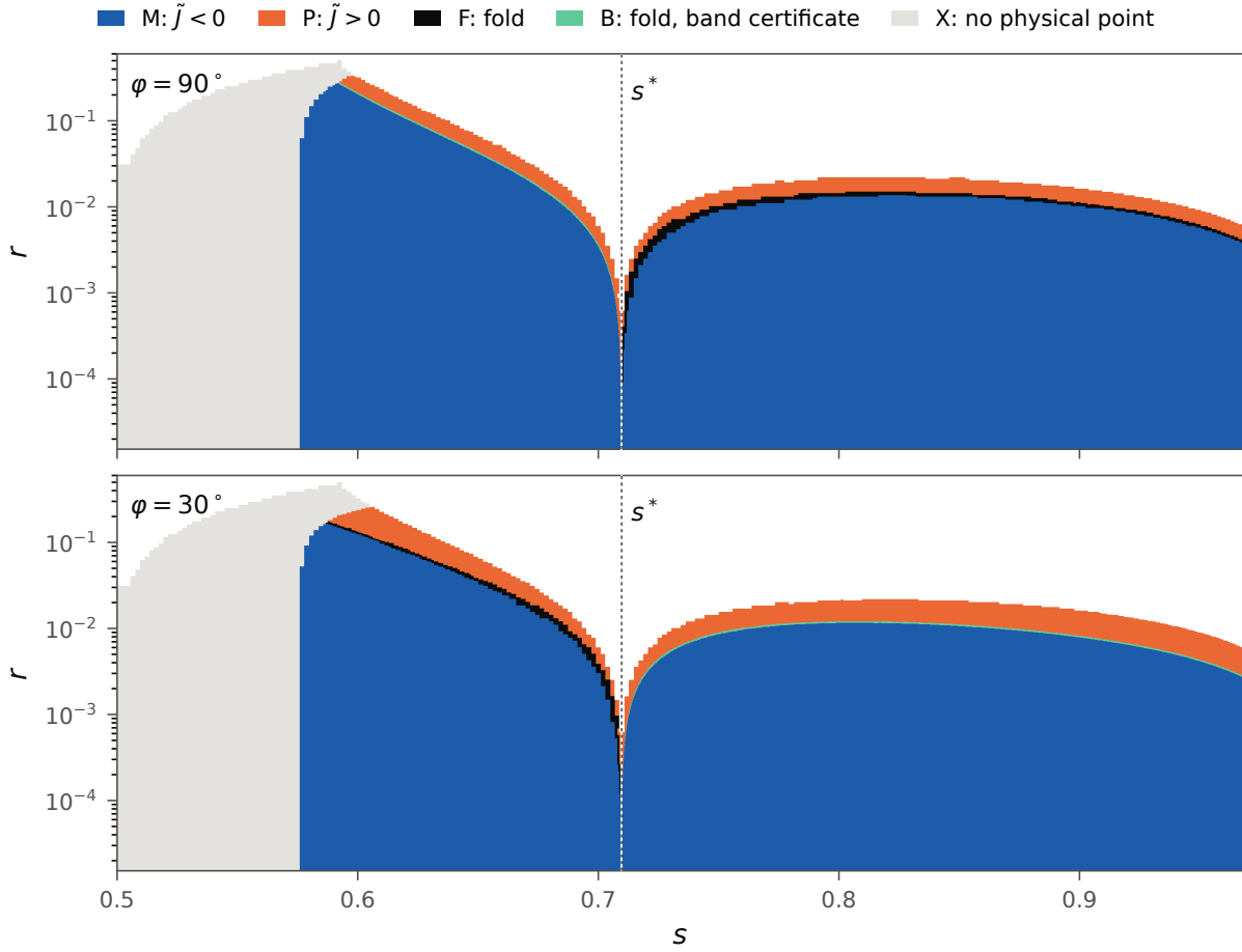
FIGURE 3. The leaves of the core, lower core, axis and lower axis covers that meet the mirror planes \varphi = 90^\circ (top) and \varphi = 30^\circ (bottom), drawn in the (s, r) -plane with r on a logarithmic scale and coloured by type (Table 4). The leaves of type U, which lie in the umbilic ball, are not drawn. The legend gives the certified signs of \tilde{J} = (-K)J , which are those of J at the physical points (Lemma 3.1(a)). Leaves of type B, which are thinner than a line at this scale, are drawn one line high. The leaves of type M reach the bottom edge of the plot, r = 2^{-16} . They lie below the fold, except for s below about 0.59, where the rays in the mirror planes do not meet the fold (case (R2) of Corollary 6.9) and the leaves of type M lie directly below leaves of type X. Those of type X on the left contain no physical point: physical points have s > 1/\sqrt{3} (Lemma 4.2). The leaves of type X above the others, for s < 0.61 , contain no physical point either. They have K > 0 or are excluded by the \alpha -test (Table 3). For s \geq 19/32 the region above the drawn leaves is that of the bulk cover, where J > 0 . For s < 19/32 no physical point lies above r = \sqrt{6}(2s - 1) (Lemma 4.1). Neither the zone column around s^* , covered by the umbilic cover and narrower than the dotted line at s^* , nor the strip s \geq 31/32 , covered by the top covers, is drawn. Near s = s^* the band of leaves of types F and B descends towards the axis until it reaches the edges of the zone column, where its lowest leaves lie at about r = 10^{-4} ; inside this column the fold reaches the axis at p^* , where \bar{D} splits into the two nappes.
