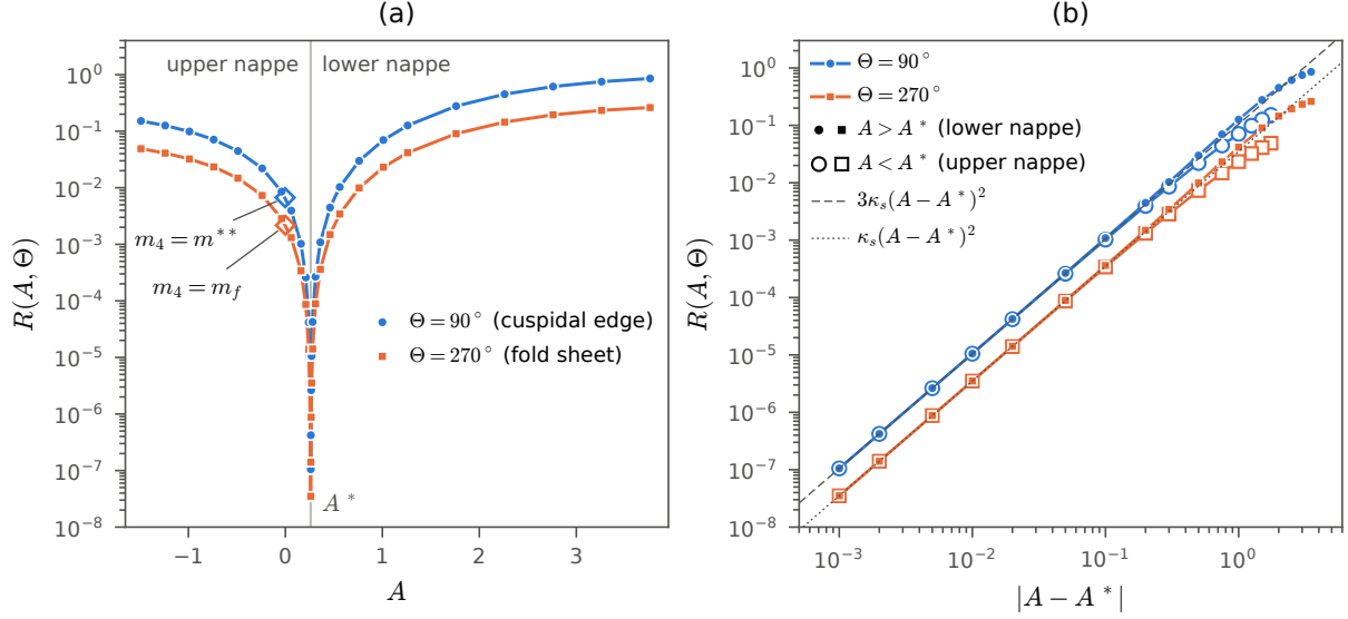
FIGURE 1. The surface of critical values \rho = R(A, \Theta) of Theorem 1 on the mirror rays \Theta = 90^\circ (cuspidal edge) and \Theta = 270^\circ (fold sheet), at 32 levels of A from A^* - 1.75 to A^* + 3.5 , against A , with R on a logarithmic axis (a), and against |A - A^*| on logarithmic axes (b). The marks are circles on the ray \Theta = 90^\circ and squares on the ray \Theta = 270^\circ . In (b) they are filled on the lower nappe ( A > A^* ) and open on the upper nappe ( A < A^* ). In (a) the ten levels with |A - A^*| \leq 0.02 crowd near A^* , where their marks overlap; (b) separates them. All plotted values of R are certified enclosures, of radius less than 10^{-71} , from the mirror system of Section 9.1. The lines between the levels are drawn for the eye. The values of R at the other angles, which are known only in floating point, are not shown. The reference lines in (b) are 3\kappa_s(A - A^*)^2 and \kappa_s(A - A^*)^2 , where \kappa_s = 0.0351137\dots is computed from the closed forms of Propositions 2.4 and 2.6. They are the asymptotic radii on the two rays as A \rightarrow A^* (Proposition 12.1). Near A^* the plotted values lie close to them. The open diamonds in (a) are the mass coordinates of body 1 for the masses (1, 1, 1, m^{**}) and (1, 1, 1, m_f) , which lie on the surface (Corollary 10.7).
