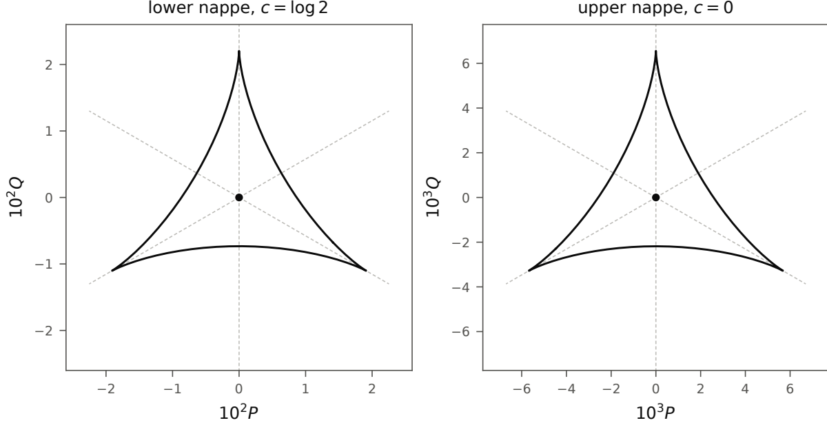
FIGURE 2. The curves C_c = G(\Gamma_c) for c = \log 2 on the lower nappe (left) and c = 0 on the upper nappe (right), computed in floating point. The dot is the origin, the image of the axis point of the disk \Phi_c . This point has m_4/m = 1/2 on the left. On the right it is the equilateral configuration of four equal masses. The dashed lines are the mirror rays \Theta = 30^\circ + k \cdot 60^\circ . Each curve meets every ray from the origin once. It has cusps on the mirror rays \Theta = 90^\circ, 210^\circ and 330^\circ and crosses the other three mirror rays transversally, as Proposition 7.13 shows for all levels c \neq A^* . The two curves look alike, but the cusp points of \Gamma_c lie on the half-mirrors \varphi \in \{90^\circ, 210^\circ, 330^\circ\} on the lower nappe and on \varphi \in \{30^\circ, 150^\circ, 270^\circ\} on the upper nappe.
